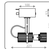
PHIL53 SK RETAKA - halogen12V 50W (100mm) anod* 63170120 silver* 63170122 - CDM-Rm 35W (100mm) anod* 63180120 silver* 63180122
