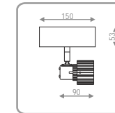
PHIL53 SO MAXI STAR TECHNO - halogen230V 50W anod.* 62200120 silver* 62200122 - halogen12V 50W anod.* 62220120 silver* 62220122 - CDM-Rm 35W anod.* 62240120 silver* 62240122
