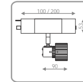
PHIL53 SK MAXI STAR TECHNO - halogen230V 50W (100mm) anod* 63190120 silver* 63190122 - halogen12V 50W (200mm) anod* 63200120 silver* 63200122 - CDM-Rm 35W (200mm) anod* 63210120 silver* 63210122
